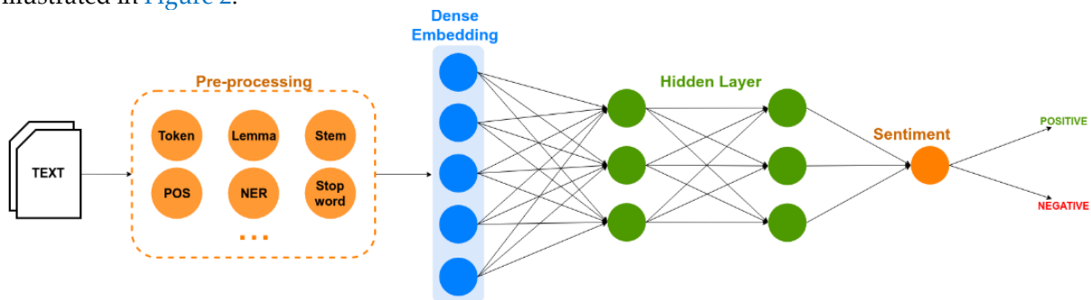
Figure 2. Deep learning.
